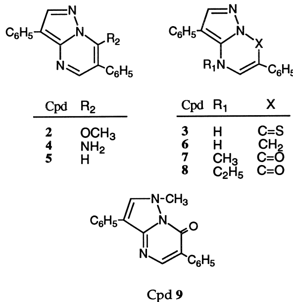
Figure 3. Molecular formulas of compounds 2–9.
