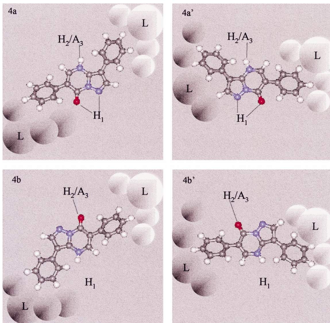
Figure 4. Schematic representation of four possible orientations (4a, 4a'; 4b, 4b') of compound 1 respect to BZR.
