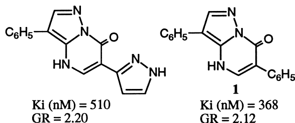
Figure 2. Molecular formulas and biological data of lead molecules.
