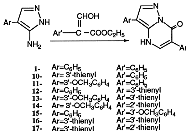
Scheme 1. One-step reaction for the synthesis of compounds 1 and 10–17 .
