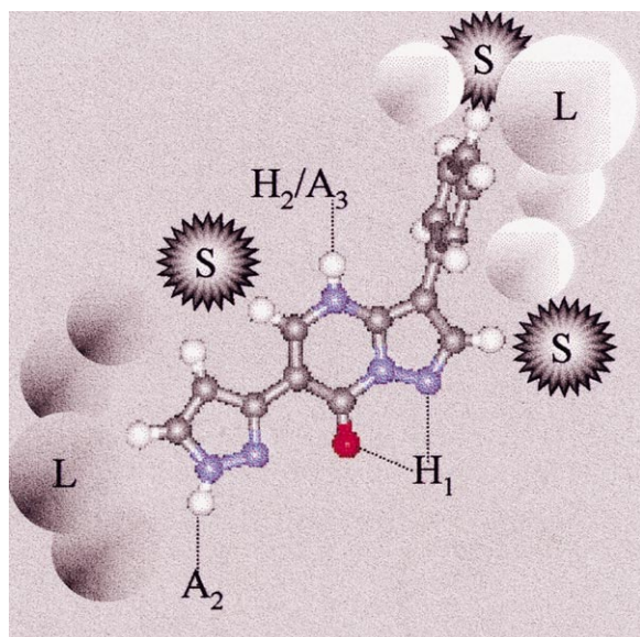
Figure 1. Schematic representation of the interaction between 4,7-dihydro-3-phenyl-6-pyrazol-3'-yl-pyrazolo[1,5-a]pyrimidin-7-one (lead compound) and BZR.
